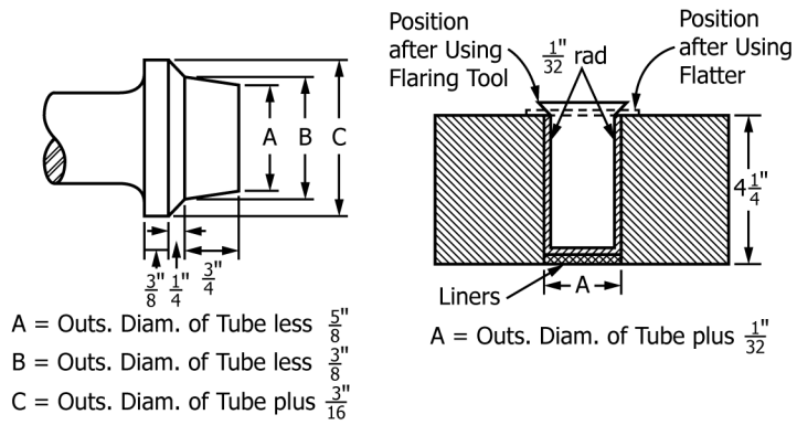
Flaring Tool
