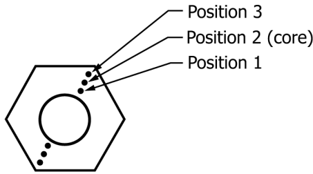
FIG. A3.7 Hardness Test Indentation Locations
